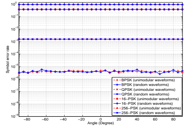
Fig. 4. SER versus spatial angle of the communication receiver.
