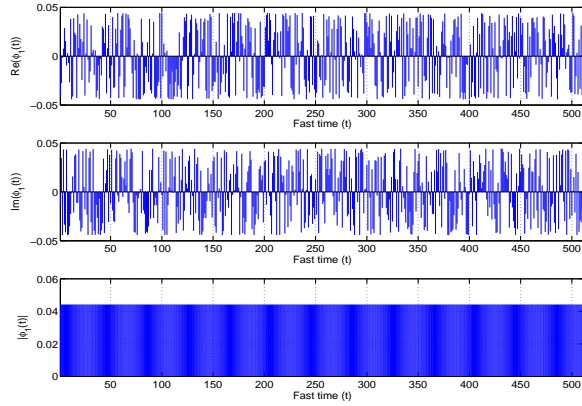
Fig. 2. Real-part, imaginary-part, and magnitude of \phi_1(t) ; unimodular waveform.
